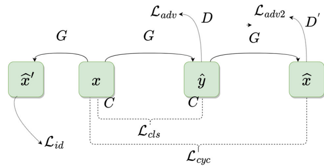
Fig. 4 The training strategy of StarDance, which involves five types of losses: adversarial loss \mathcal{L}_{adv} , cycle-consistency loss \mathcal{L}_{cyc} , identity-mapping loss \mathcal{L}_{id} , second adversarial loss \mathcal{L}_{adv2} , and domain classification loss \mathcal{L}_{cls} . See Sect. 3.3 for the definition of notations
